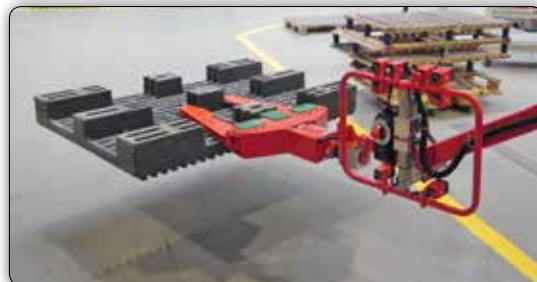
Manipulator with forks tooling for handling pallets.
