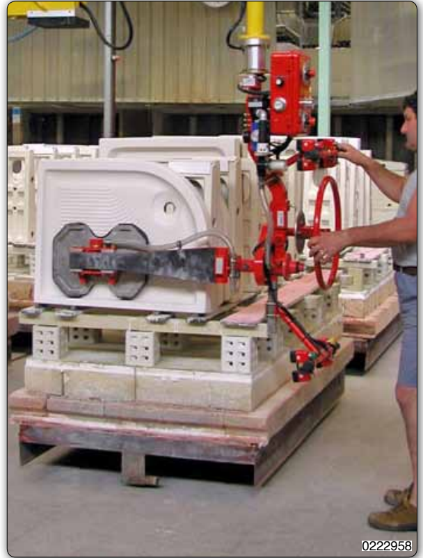
PMF Partner manipulator, fixed overhead, with suction cups tooling (Venturi) for gripping and manual rotation of shower plates.
