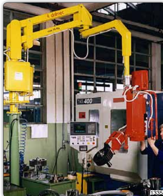
PMC type Partner manipulator, column design, with special equipment for picking, inclination and rotation of gears.
