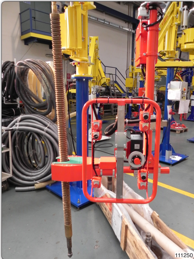
Manipulator with pneumatic tooling for gripping and handling shafts.
