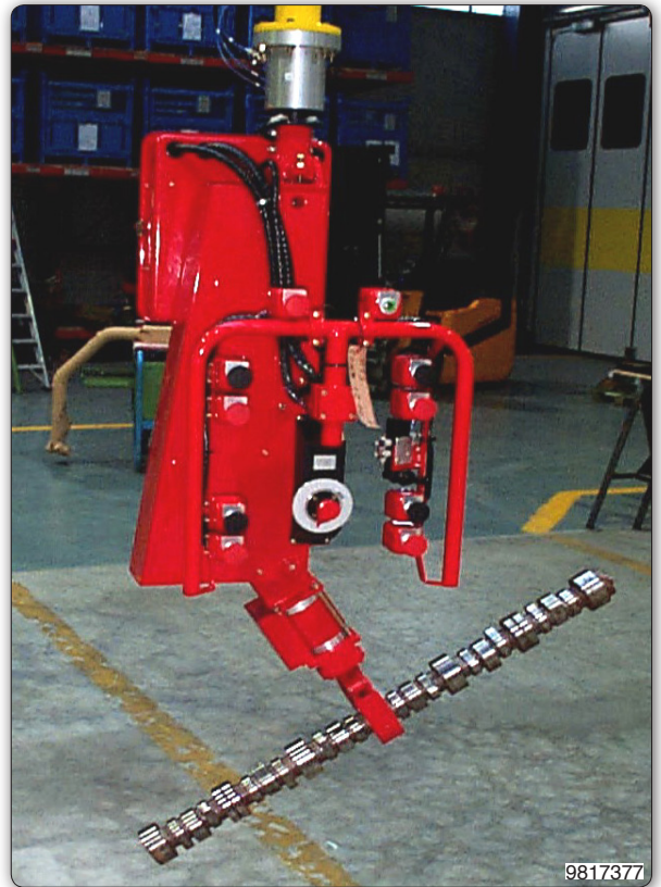
Manipulator with pneumatic tooling for gripping and inclination of mechanical shafts.
