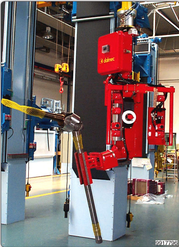
Manipulator with pneumatic tooling for gripping, inclination and rotation of transmission shafts.
