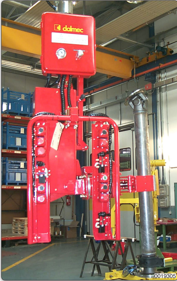
Manipulator with jaws tooling for gripping and rotation of transmission shafts.
