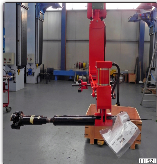
Manipulator with pneumatic tooling for gripping and inclination of shafts.
